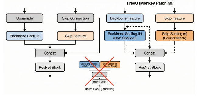
Figure 1. Comparison between Naive Hook and our Dynamic Monkey-Patching strategy. Standard hooks intercept features too late (after concatenation), whereas Monkey-Patching allows for precise modulation prior to the concatenation operation.
