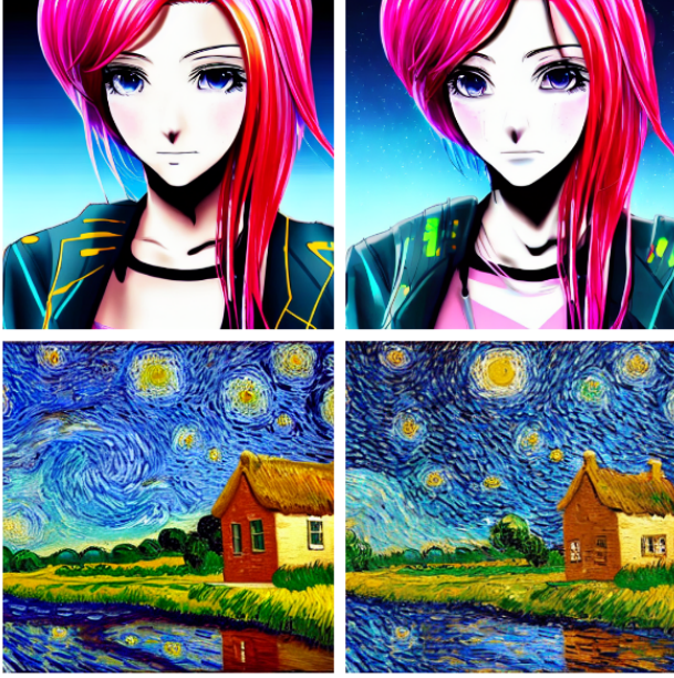
Figure 7. Comparison between Static and Dynamic FreeU across different artistic styles. Top Row (Anime): Static FreeU suffers from color oversaturation and artificial lighting. Dynamic FreeU maintains vibrant colors with natural gradients. Bottom Row (Oil Painting): Static FreeU interprets brush strokes as noise, creating jagged artifacts. Dynamic FreeU preserves the fluid, painterly texture of the Van Gogh style.
